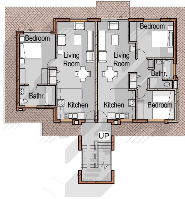
1 Ground Floor 1 : 200
